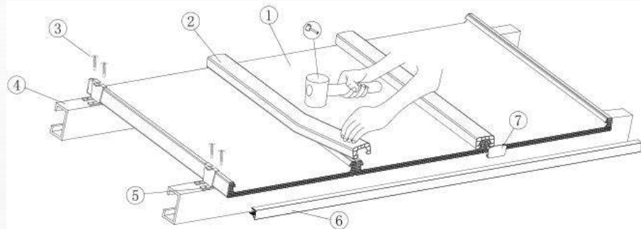
4, 安装PC或者铝合金扣条 Install the PC or AL gasket cover
